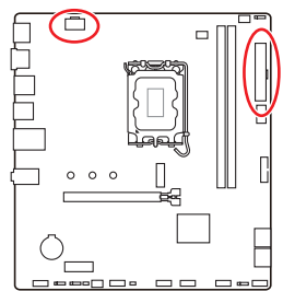
CPU_PWR1
