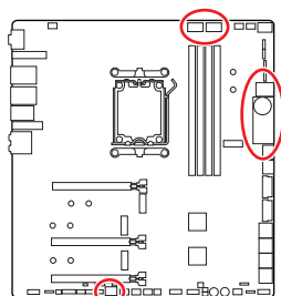
CPU_PWR1~2
