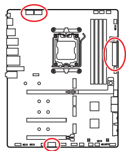
CPU_PWR1~2
