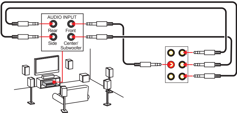
Audio jacks to 7.1-channel speakers diagram
