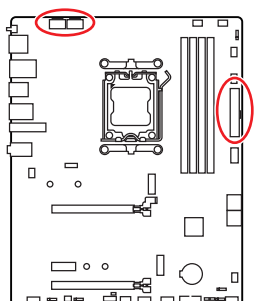
CPU_PWR1, CPU_PWR2
